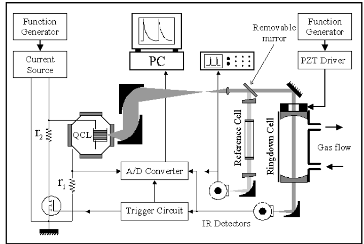
Figure 1. Schematic of a CRDS based gas sensor schematic. 4 r_1 - current monitor resistor; r_2 - current-limiting resistor. Two wedged ZnSe windows shown near the reference cell were used to form an etalon for fine frequency calibration.
