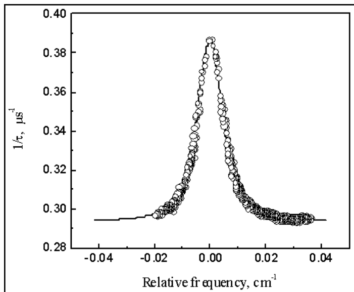
Figure 3. CRDS spectrum of NO in N_2 , unresolved lines at 1921.599\text{ cm}^{-1} and 1921.601\text{ cm}^{-1} . The solid line shows a Voigt fit, which resulted in NO concentration of 622 ppbv.
