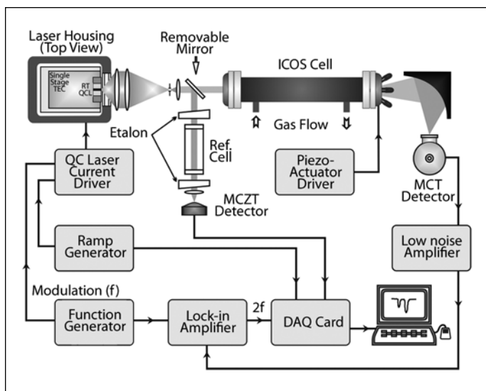
Figure 1. TEC-CW-DFB QCL based OA-ICOS sensor. MCT is a cryogenically-cooled photovoltaic HgCdTe detector, and MCZT is a thermoelectrically-cooled HgCdZnTe photodetector (Vigo System, Model PVMI-10.6).
